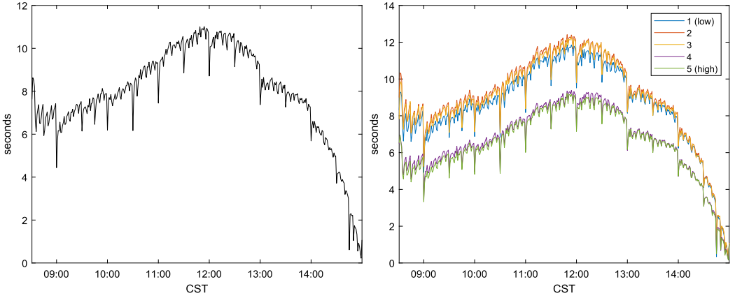
FIGURE S2. Staleness of prices. The left figure plots the cross-sectionally averaged average staleness. The right figure plots the average staleness for prices of stocks sorted according to their beta at market open.
