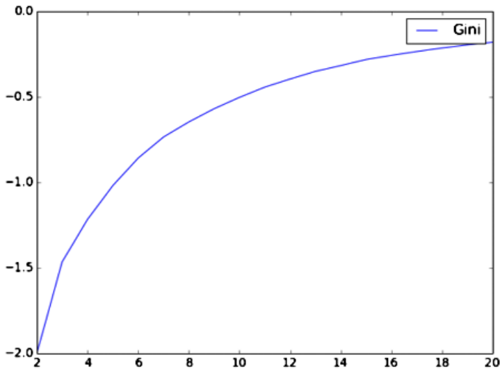
FIGURE 1. Gini coefficient.
