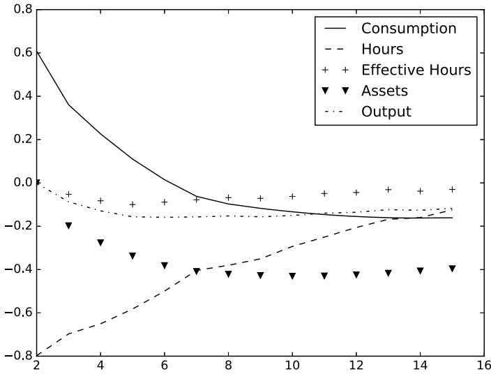
FIGURE 2. Aggregate variables.
