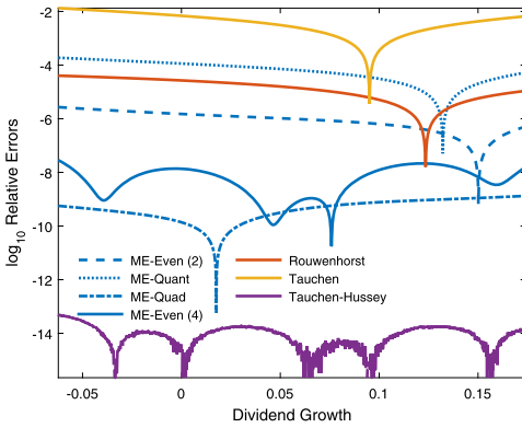
(c) N = 15 .
