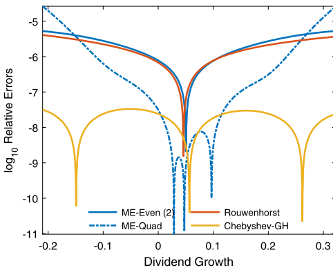
(c) \rho = 0.95 .
