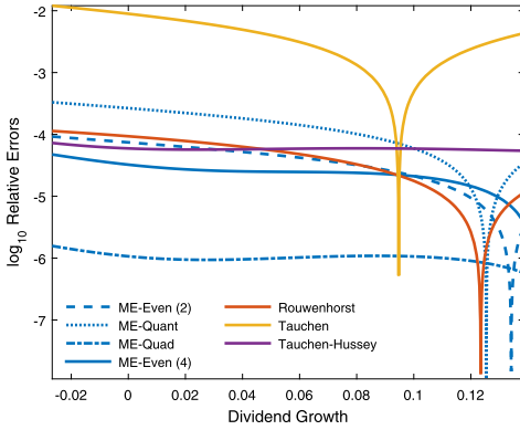
(a) N = 5 .
