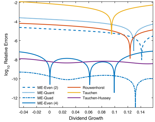
(b) N = 9 .
