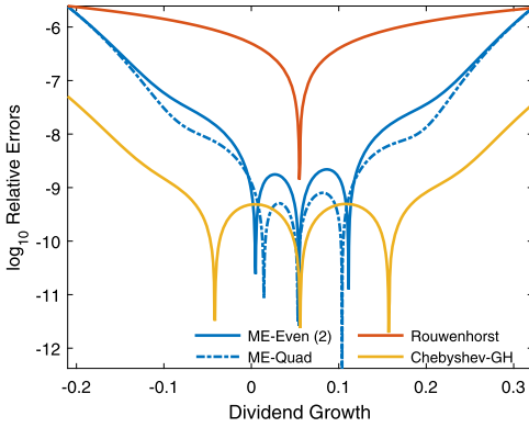
(a) \rho = 0.8 .
