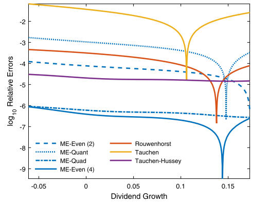
(b) \rho = 0.6 .
