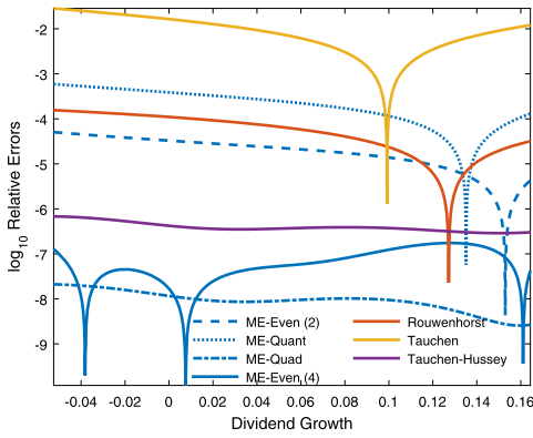
(a) \rho = 0.5 .
