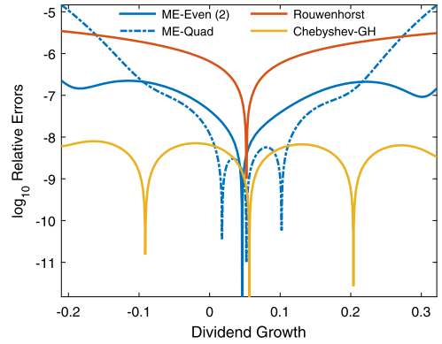
(b) \rho = 0.9 .
